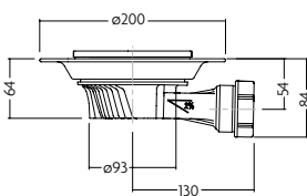
Tiled Drain Slim+ Horizontal Slot Code: SLW2T01/H Price: £267.80 Exc. VAT £321.36 Inc. VAT*
