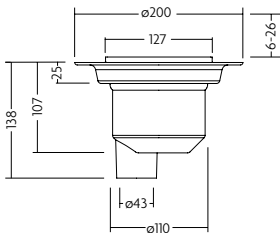
Quad Gravity Drain Slot - Vertical Outlet Code: UTT01/V Price: £183.84 Exc. VAT £220.61 Inc. VAT*
