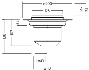
Quad Gravity Drain Tiled Insert 14mm - Vertical Outlet Code: QUADT14/V
