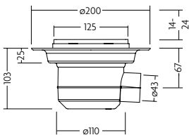
Quad Gravity Drain Tiled Insert 14mm - Horizontal Outlet Code: QUADT14/H
