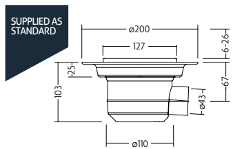
Quad Gravity Drain Slot - Horizontal Outlet Code: UTT01/H Price: £183.84 Exc. VAT £220.61 Inc. VAT*
