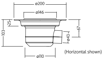
Vinyl Floor Gully - Horizontal Outlet Code: UTVCO1/H (CHROME) Price: £126.95 Exc. VAT £152.34 Inc. VAT* Code: UTVGO1/H (GREY) Price: £0.00 Exc. VAT £0.00 Inc. VAT*
