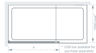
Shower Panel
